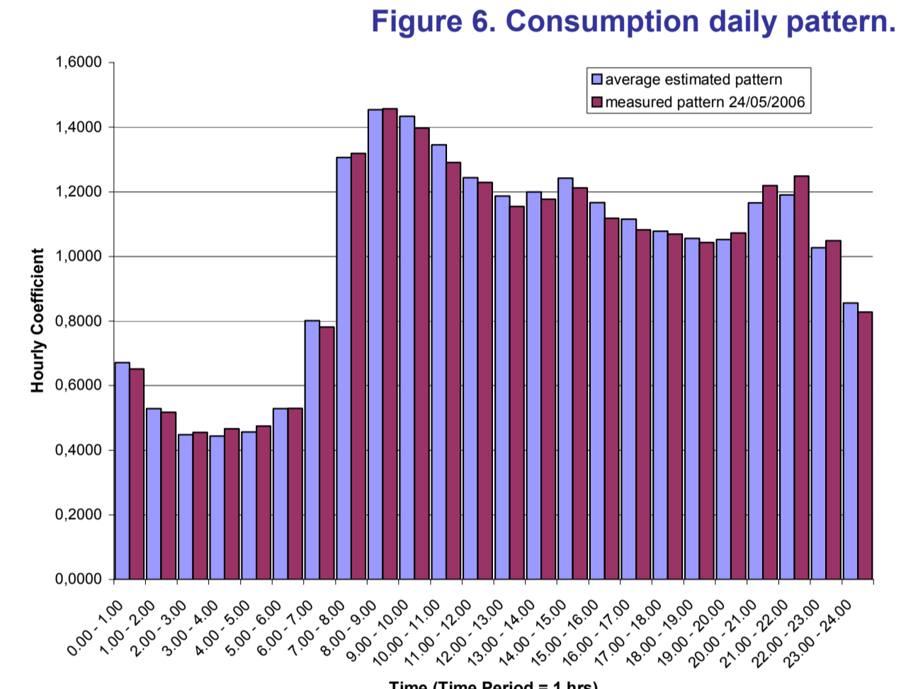
Figure 6. Consumption daily pattern.
