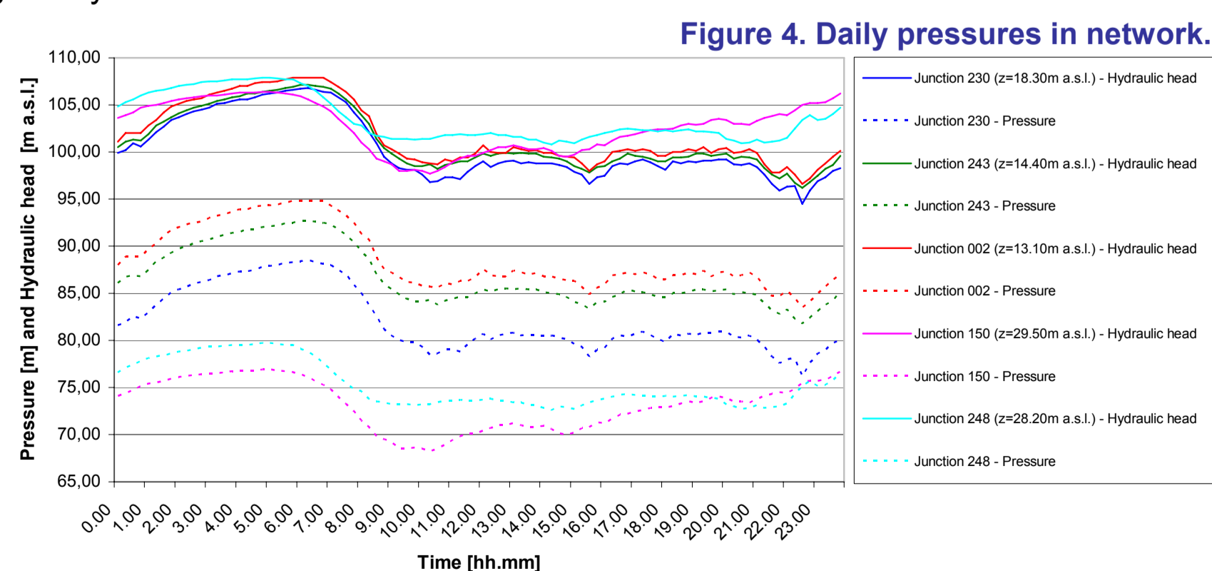
Figure 4. Daily pressures in network.
