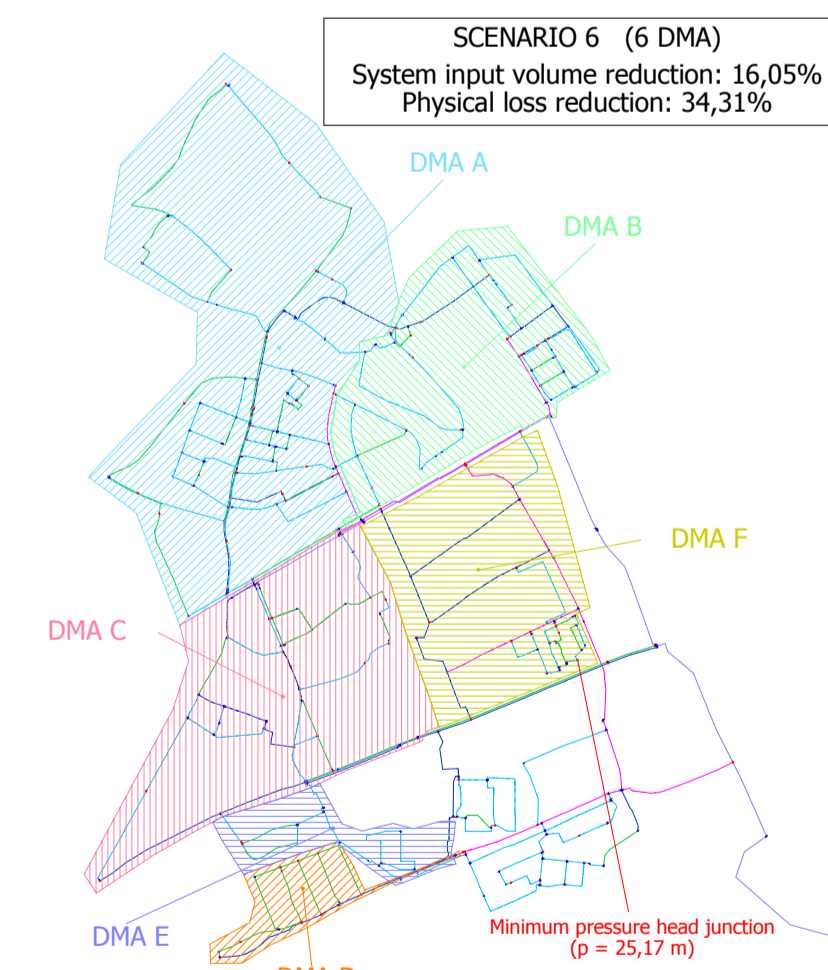
Figure 8. "Napoli Est" DMA design.
