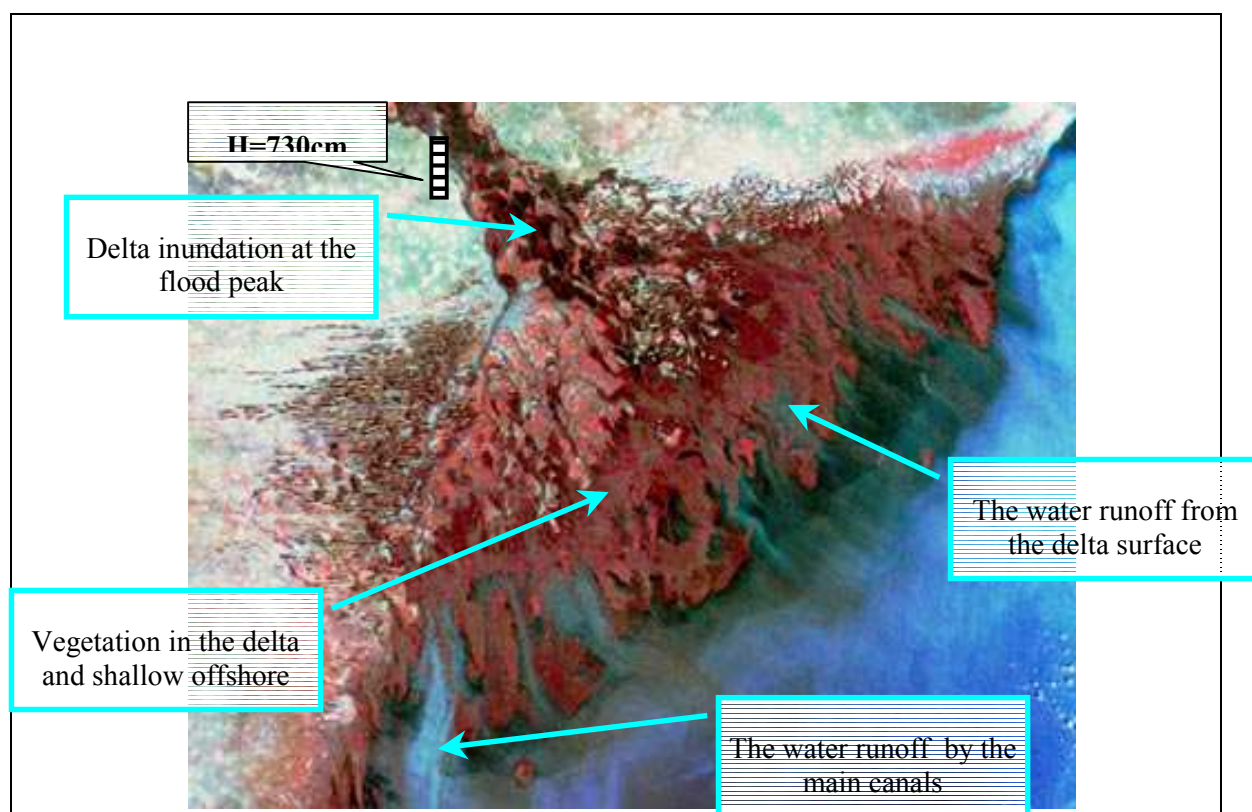
Рис. 4. Inundation during the flood peak in 2002 according to RSD
