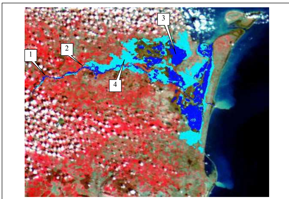
Fig. 5. Inundation of the Terek delta during catastrophic flush on the basis of RSD.
