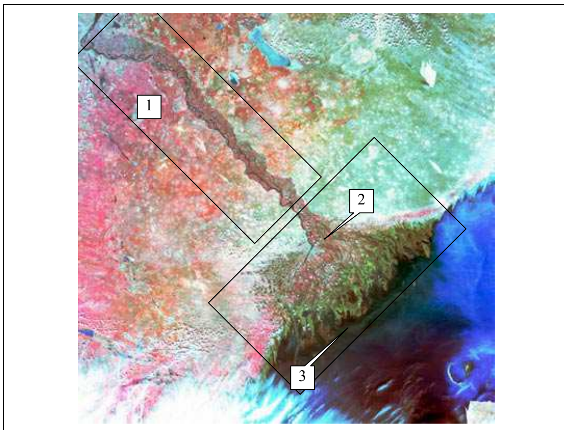
Fig. 3. Experimental Volga Region, covered with the RSD.
